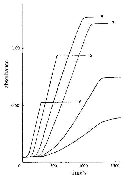
Fig. 3 Absorbance vs. time traces for the decomposition of aimsa in a basic air-saturated solution: [\text{NaOH}] = 0.05 (1), 0.1 (2), 0.2 (3), 0.5 (4), 1 (5) and 2.58 M (6); [\text{aims a}] = 1.5 \times 10^{-3} \text{ M} , 25^\circ\text{C} , \lambda = 315 \text{ nm}
